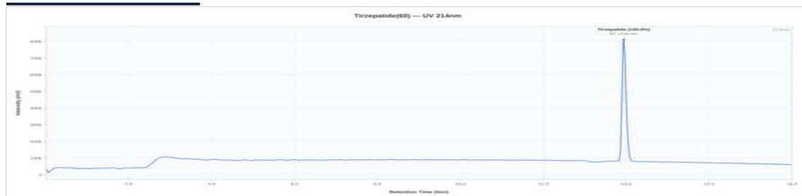
Representative chromatogram, Dedicated V0 (99.96% purity, closest to batch mean of 99.81%)
